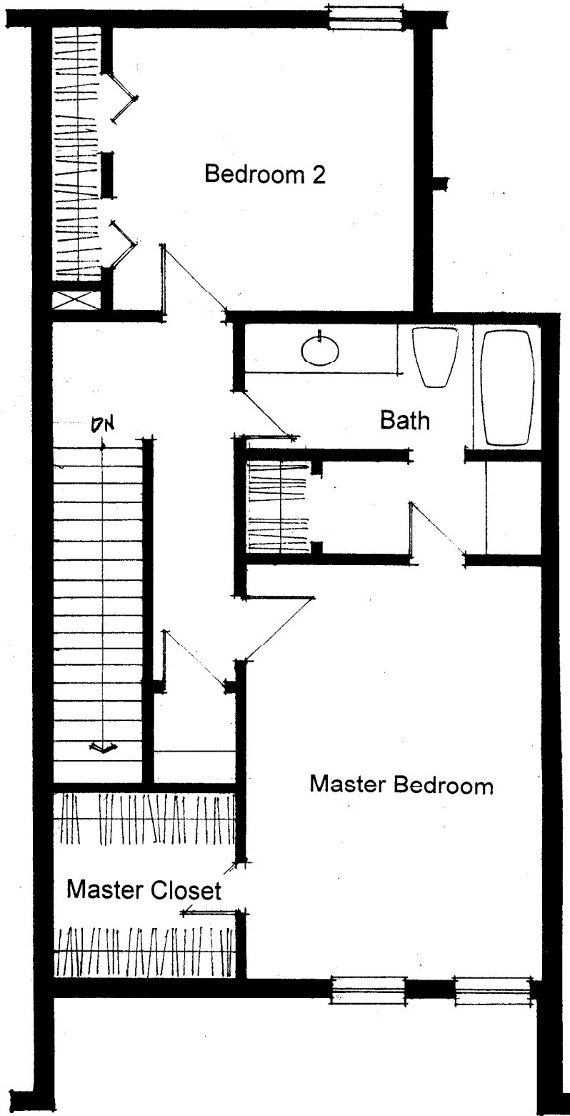
Unit F- Second Floor Plan
