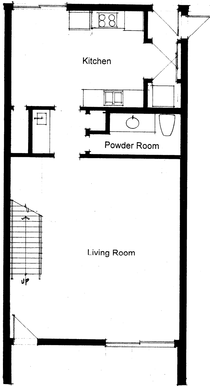
Unit F- First Floor Plan
